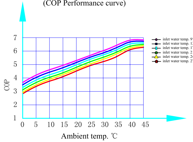
ECO-8 (COP Performance curve)
