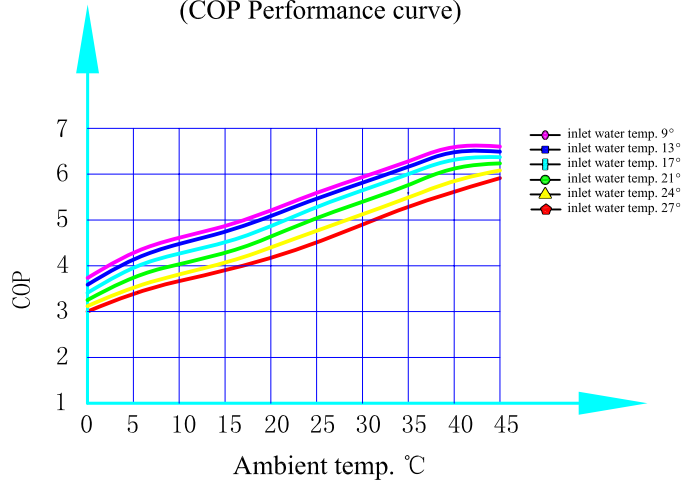
ECO-12 (COP Performance curve)
