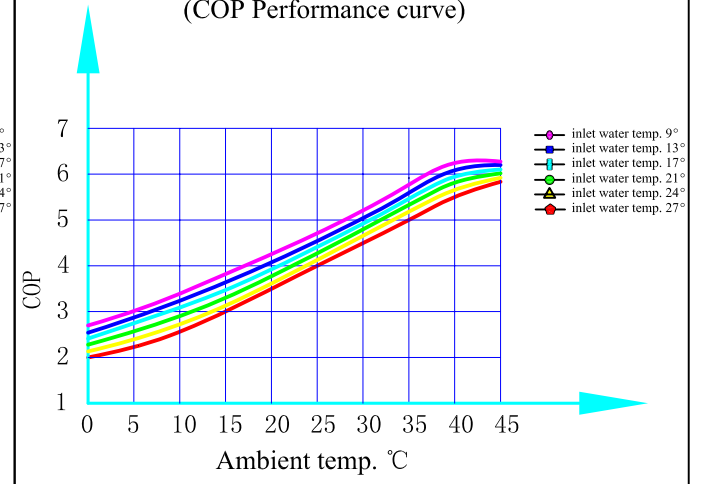
ECO-3 (COP Performance curve)
